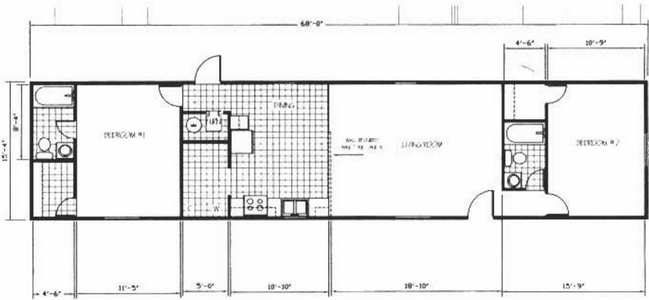
House No. 1208 16x68 2+2 EH-4 (Approx. 1042 sq. ft.)
